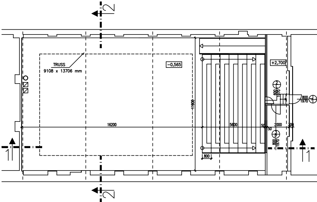
1.NP – GROUND FLOOR
